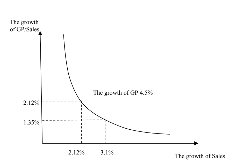
Figure 8. Decomposing GP.
